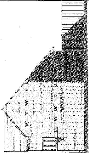
4 07.2 North - as proposed P204 1 : 100
